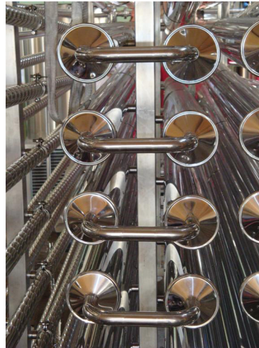
ViscoLine heat exchangers are available with different surface finish and can be electropolished if required.
