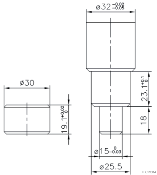
TE81B032: Fixture set f. Gear frame
