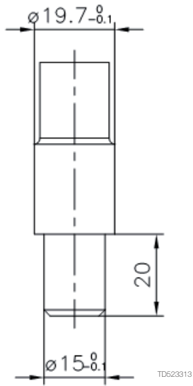
TE81B031: Pusher for Gear frame
